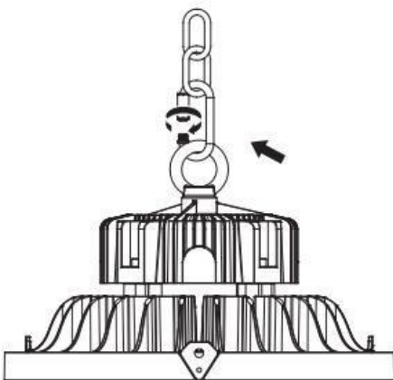
Hanging Rings
